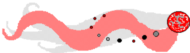
Figure 5: Lunes de Nibiru
